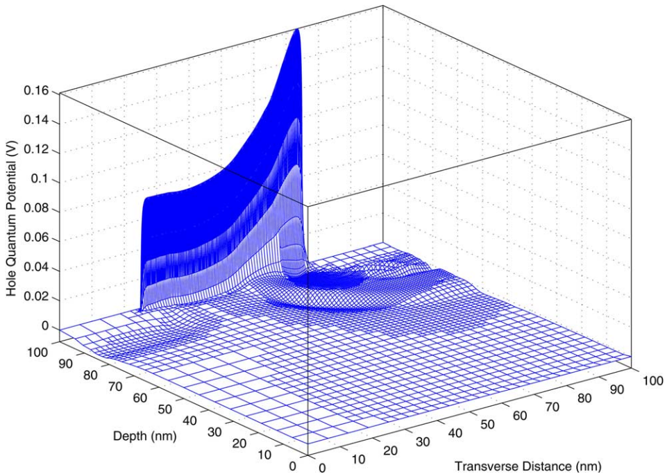
Fig. 13. Hole quantum potential.
